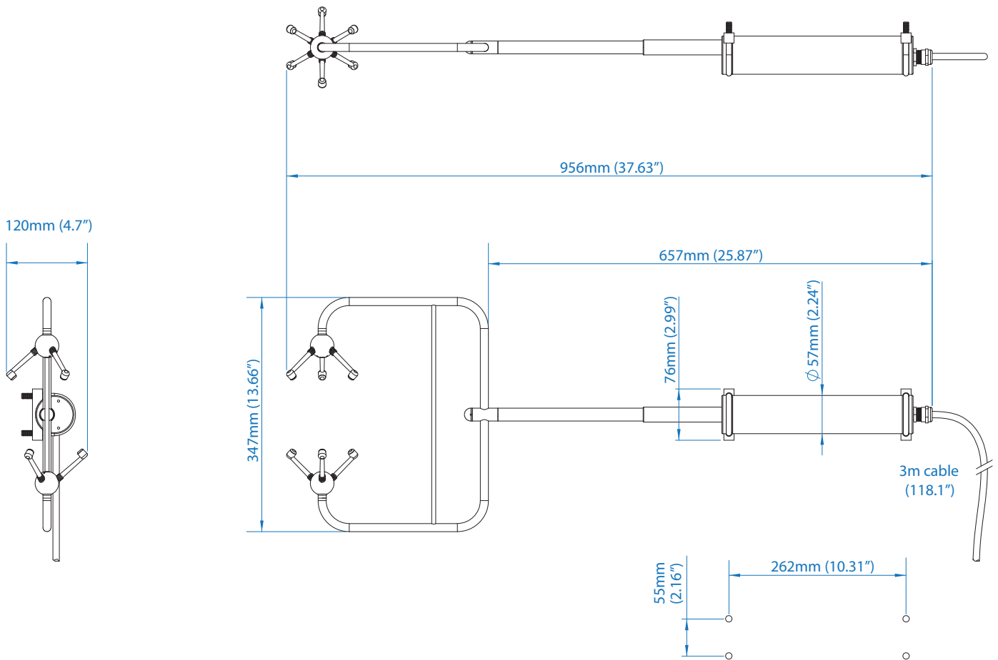
Mounting hole template for WindMaster HS 'U' Bolts 4 holes \varnothing 9.5mm (0.37") Max mounting plate thickness 5mm (0.19")
